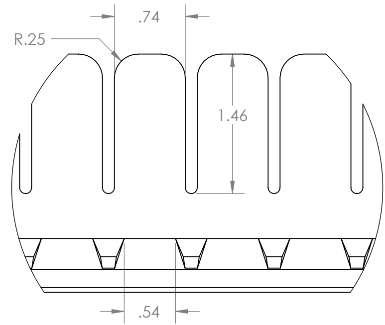
DETAIL C SCALE 1 : 1
